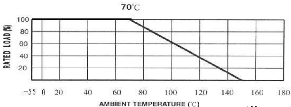
FIG.1 DERATING CURVE
